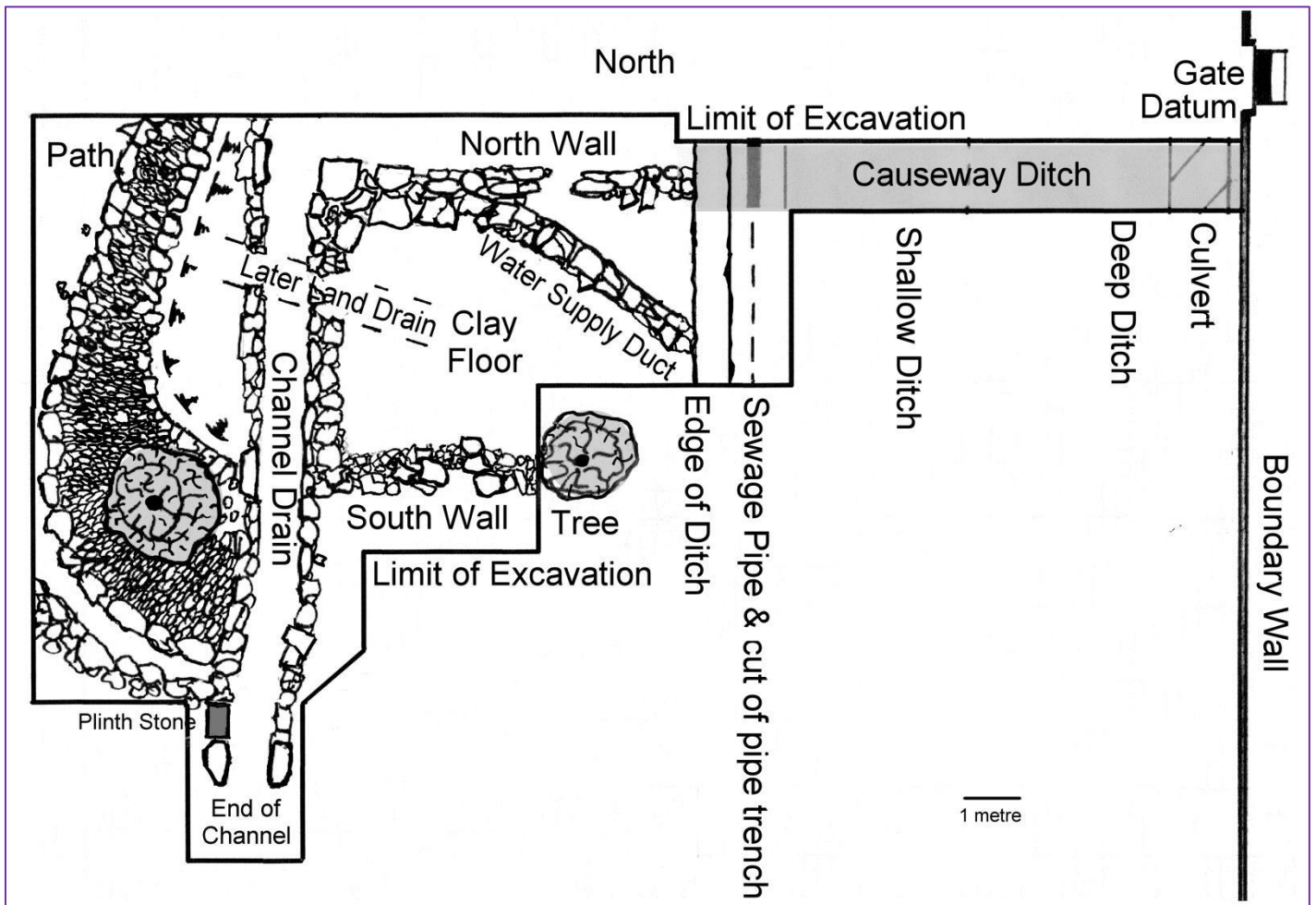
Descriptive Plan of layout of the building foundations and yard
