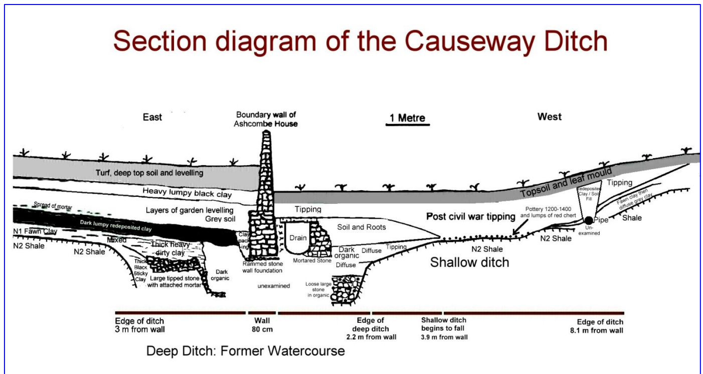
Descriptive section diagram of the Causeway Ditch and boundary wall looking south
